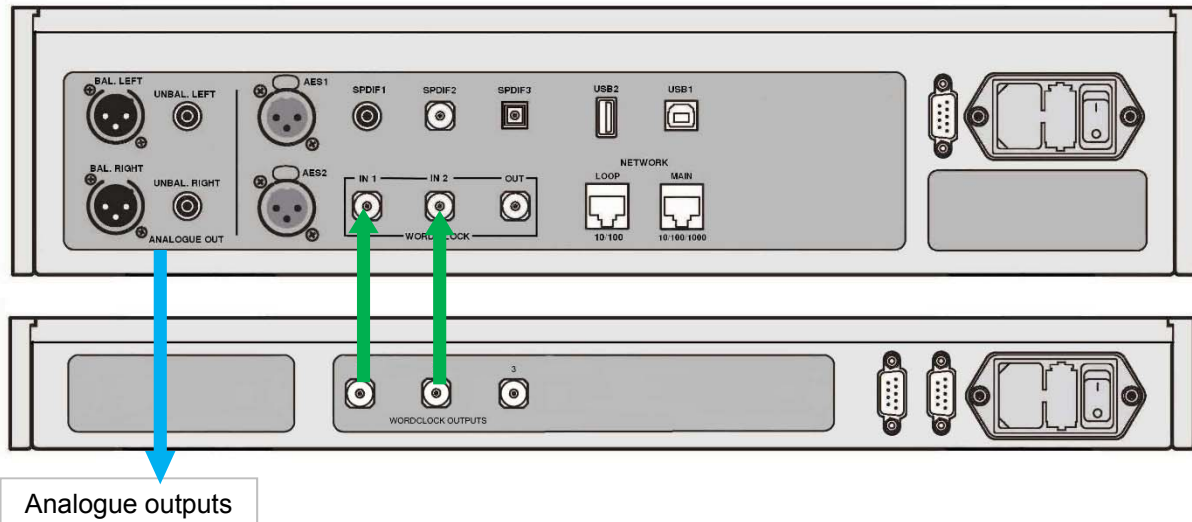
Figure 5 – Using the Bartók DAC with a Rossini Clock
